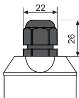
Variant "B" with short cable terminal PG11
